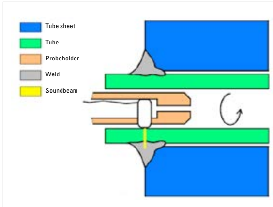
Inspection principle for using the probe to inspect a heat exchanger tube weld
